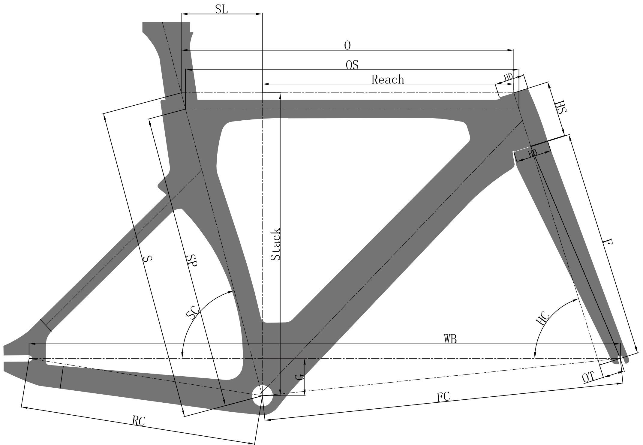
CFT126(Length:mm)
